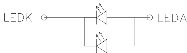
BACKLIGHT CIRCUIT
