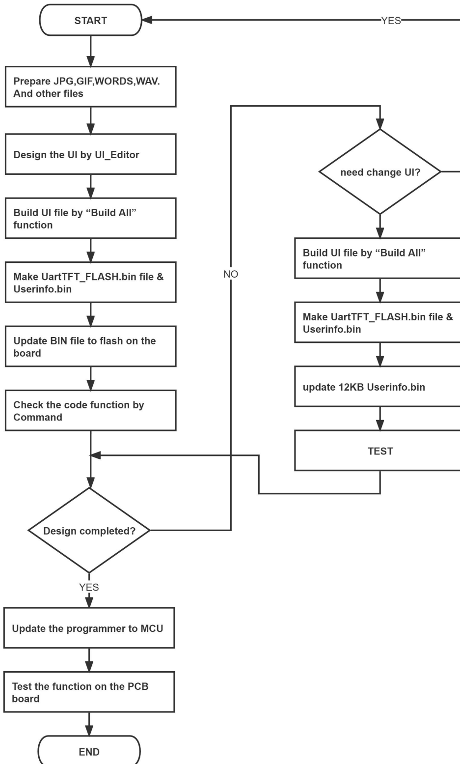
Figure 5: Design flow using UI_Editor
